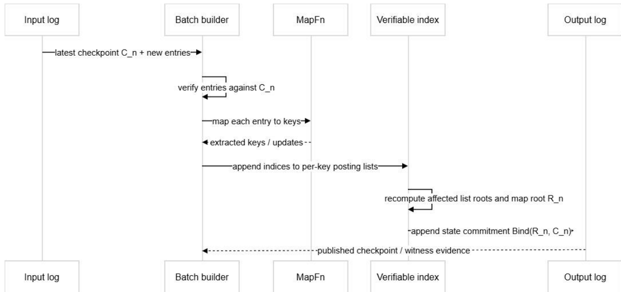
Figure 3 Verifiable Index Sequence Diagram
